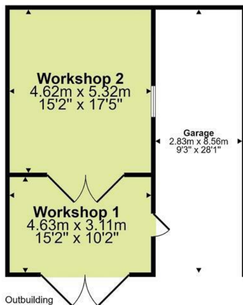
Outbuilding Approx 65 sq m / 701 sq ft
